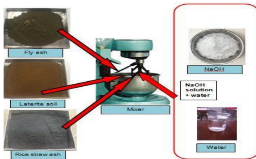
Figure 2. Mixing of geopolymers materials
